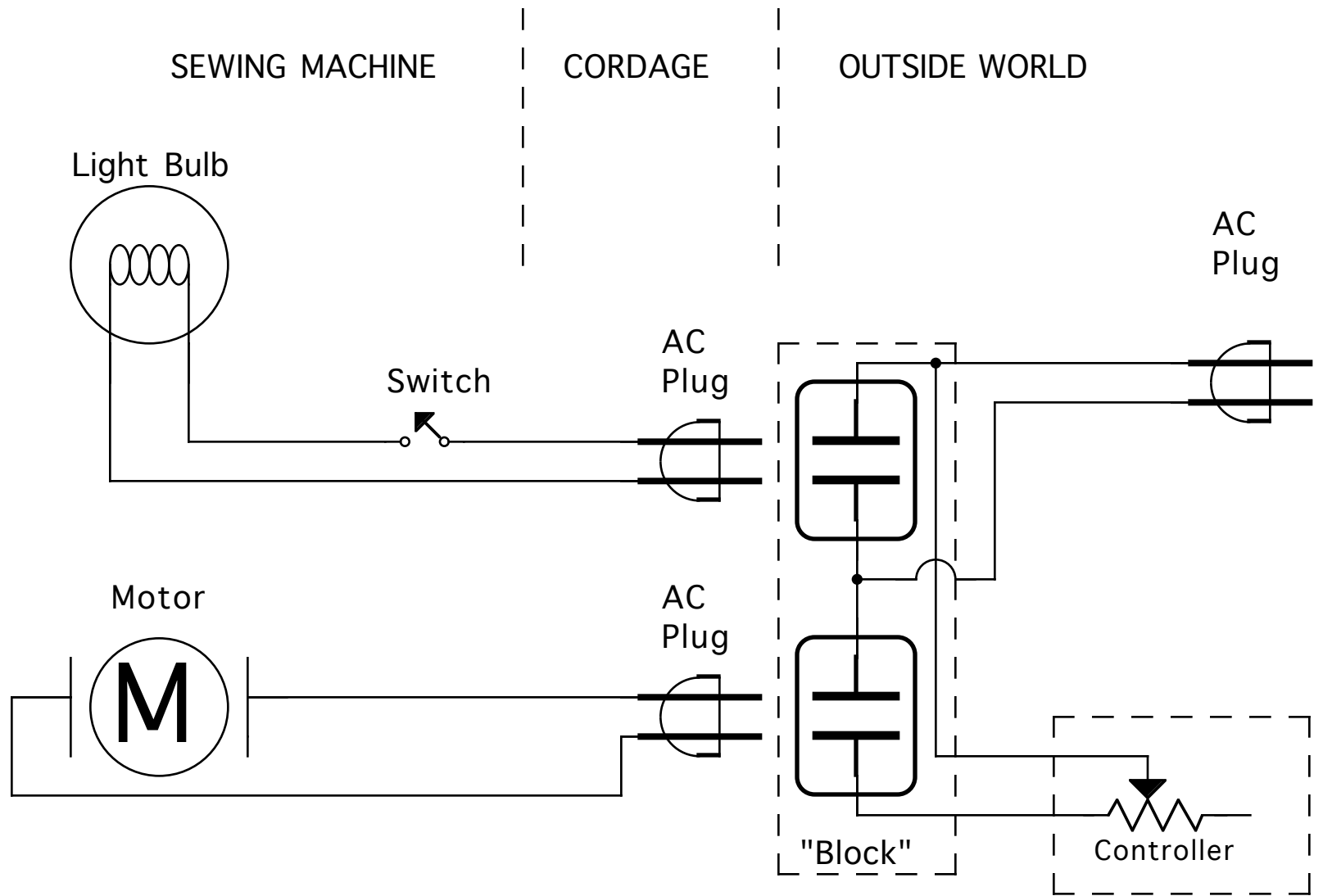
Typical Japanese Sewing Machine Wiring Diagram
