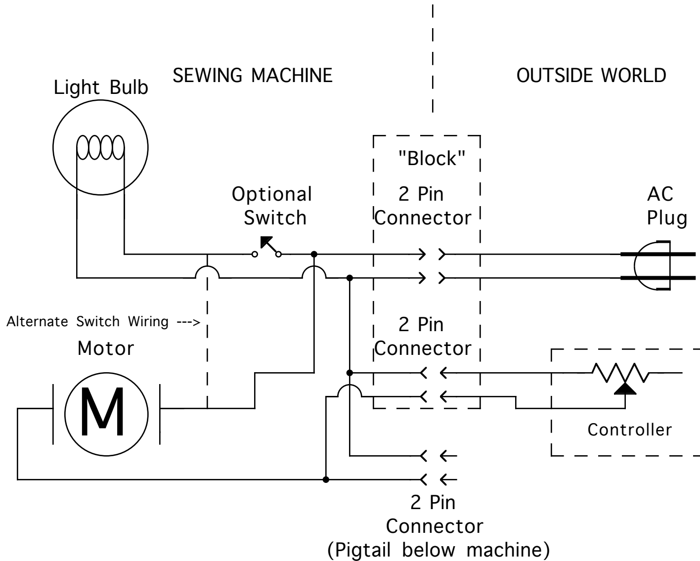
Typical NSMCo Sewing Machine Wiring Diagram
